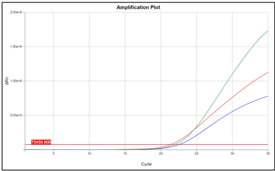
284 285 Figure 3. The amplification curve for spike (red), ori (blue), and SV40 enhancer-promoter- 286 ori (green) in a single vial of Pfizer (Lot: Fx4343a) from two different wells of the same 287 PCR run.
