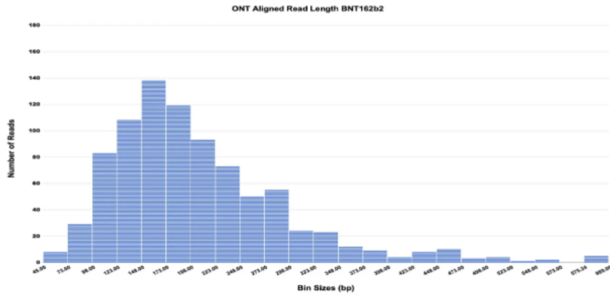
385 Figure 10. Oxford Nanopore (ONT) read length distributions from 866 reads mapped to 386 the vector sequence (NCBI OR134577.1). Mean = 214 bp. Max = 3.5 kb.
