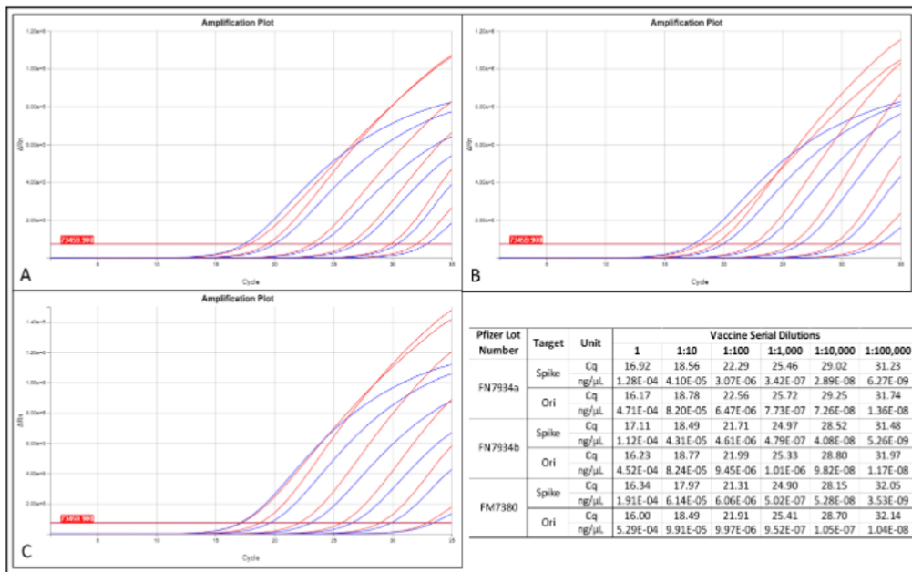
314 315 Figure 6. qPCR amplification profiles from the serial dilutions (10-fold) of the three lots 316 containing the highest DNA loads (Pfizer lots: A, FN7934a; B, FN7934b; C, FM7380).
